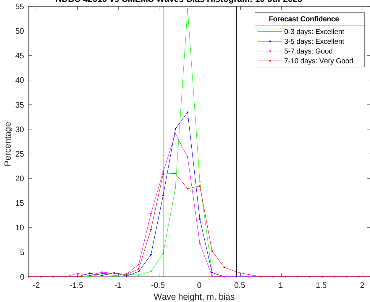
NDBC 42019 vs CMEMS Waves Bias Histogram: 10-Jul-2025
