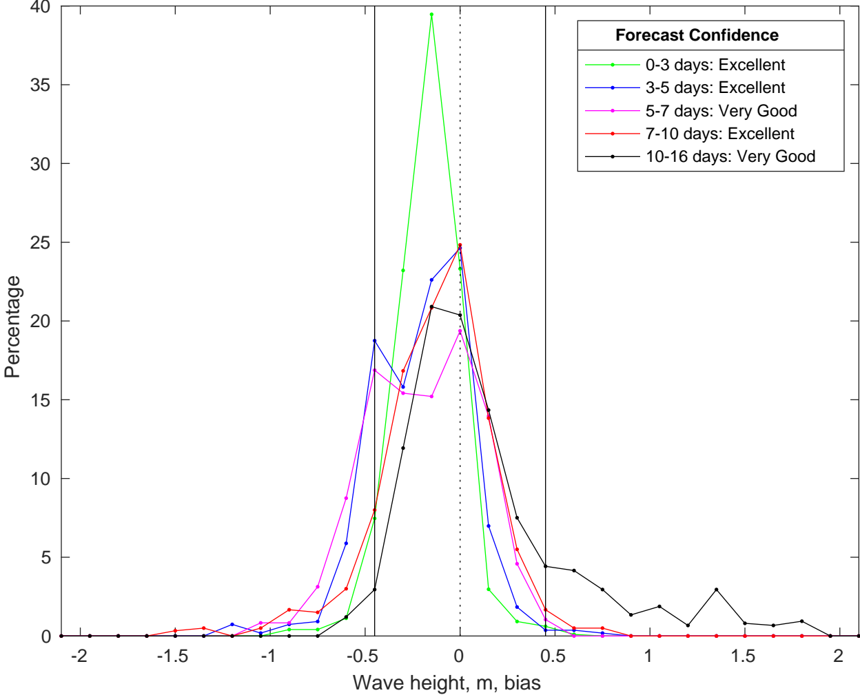
NDBC 42019 vs GFS Waves Bias Histogram: 10-Jul-2025
