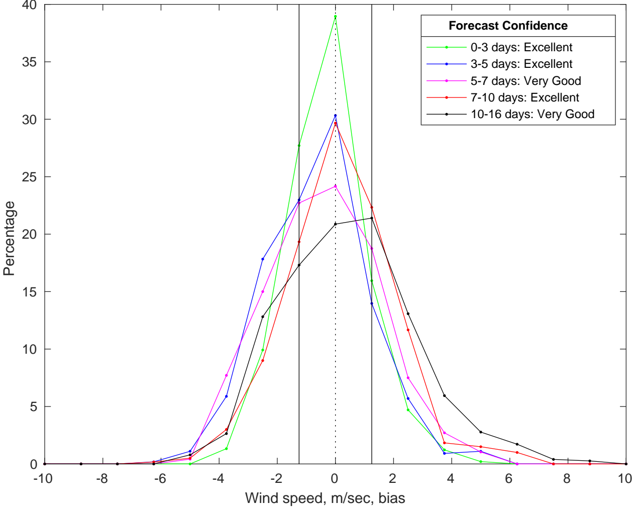
NDBC 42019 vs GFS Winds Bias Histogram: 10-Jul-2025
