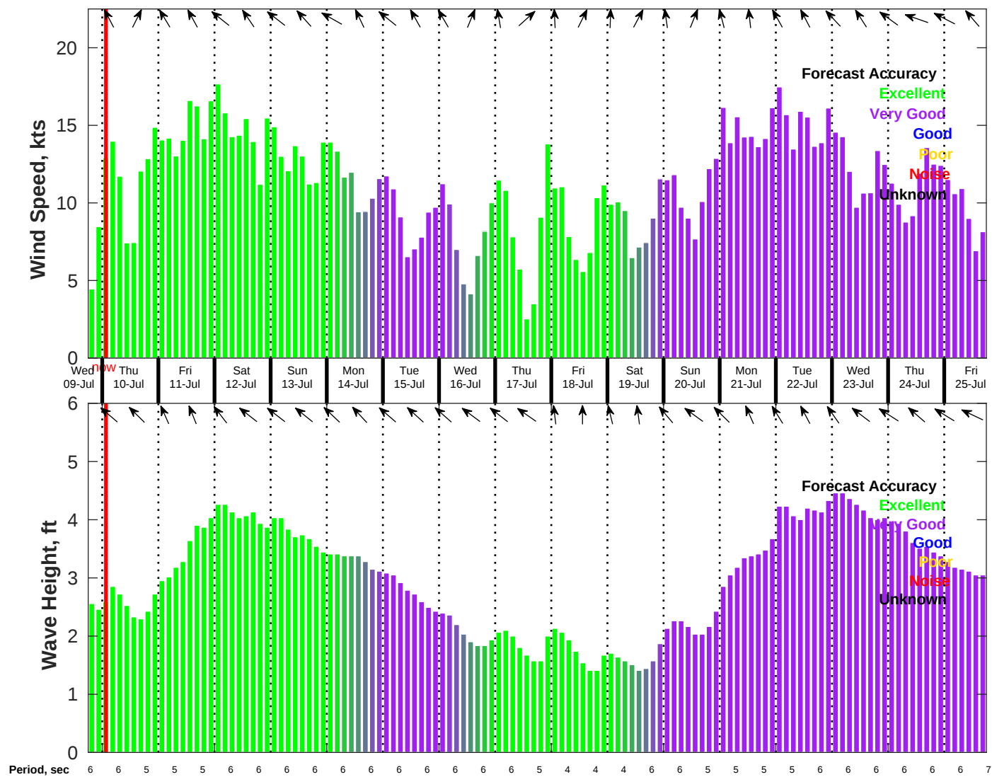
Wind & Wave Forecast for NDBC 42019 from 09-Jul-2025 18:00:00 to 25-Jul-2025 18:00:00
