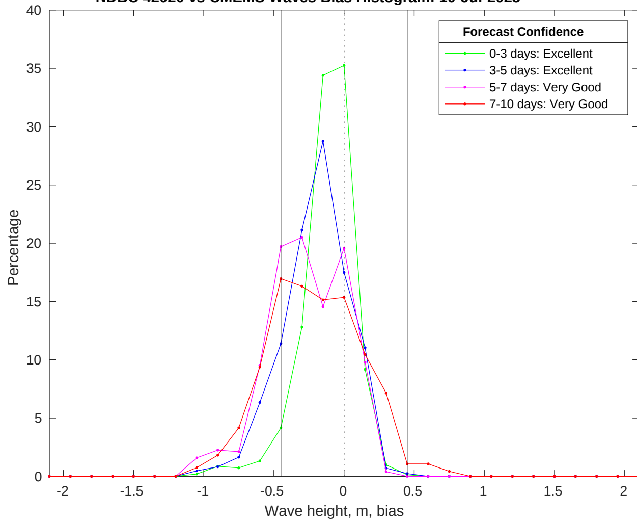
NDBC 42020 vs CMEMS Waves Bias Histogram: 10-Jul-2025
