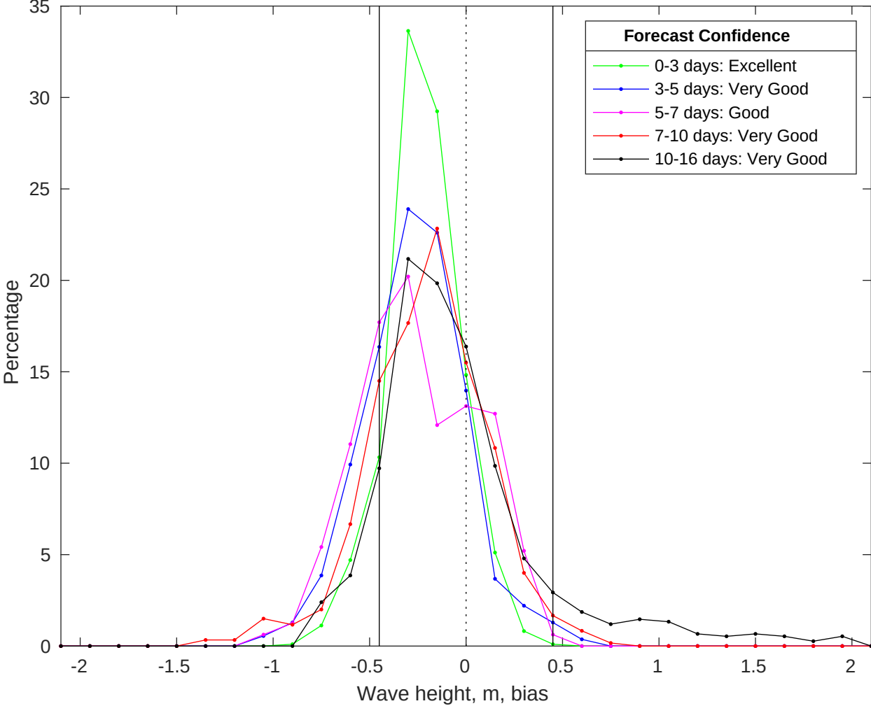
NDBC 42020 vs GFS Waves Bias Histogram: 10-Jul-2025
