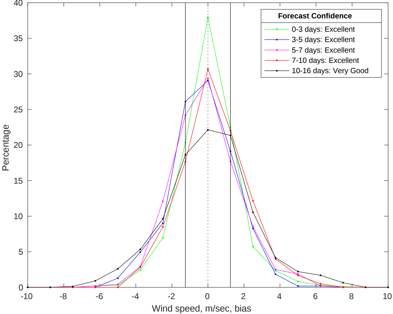
NDBC 42020 vs GFS Winds Bias Histogram: 10-Jul-2025
