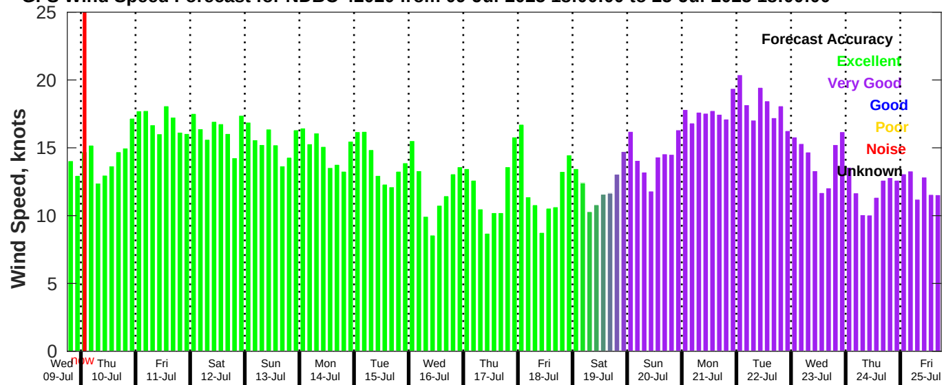
GFS Wind Speed Forecast for NDBC 42020 from 09-Jul-2025 18:00:00 to 25-Jul-2025 18:00:00
