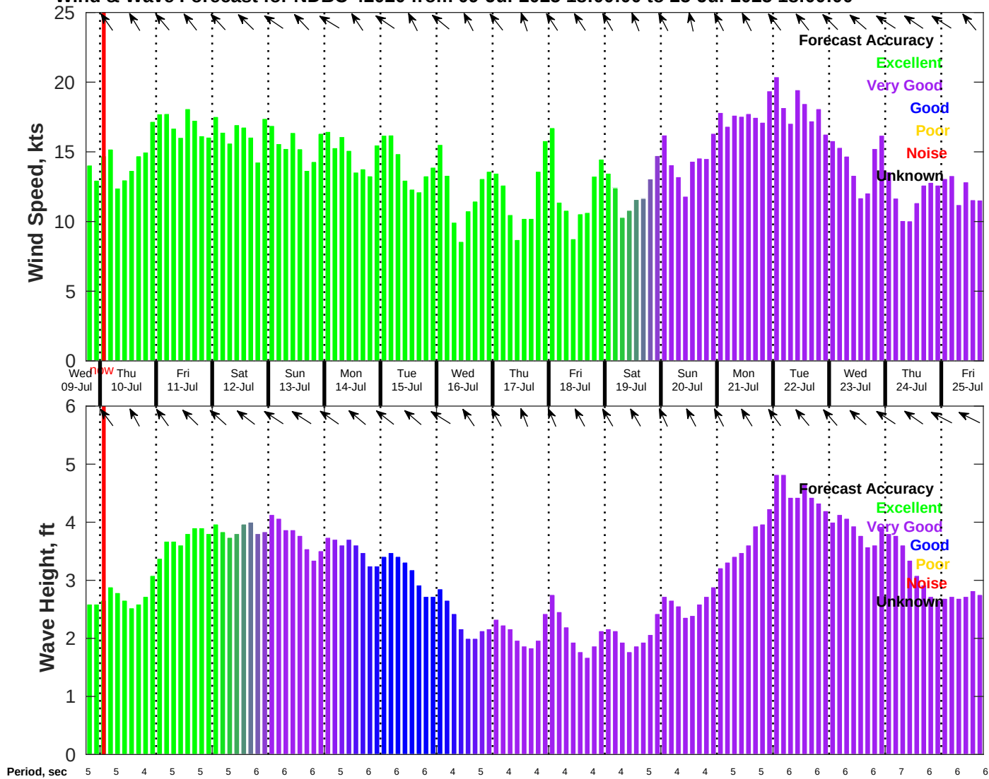
Wind & Wave Forecast for NDBC 42020 from 09-Jul-2025 18:00:00 to 25-Jul-2025 18:00:00
