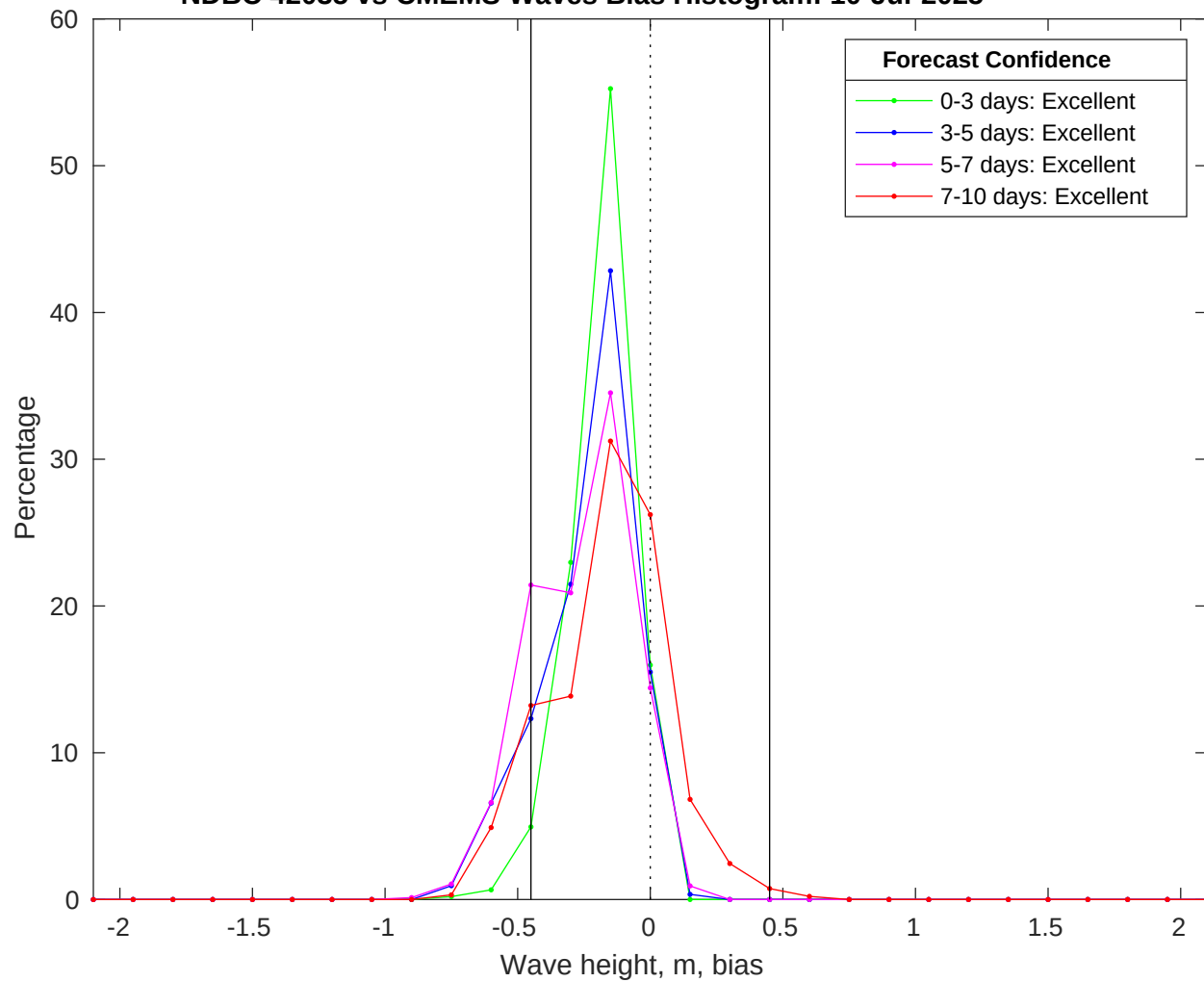
NDBC 42035 vs CMEMS Waves Bias Histogram: 10-Jul-2025
