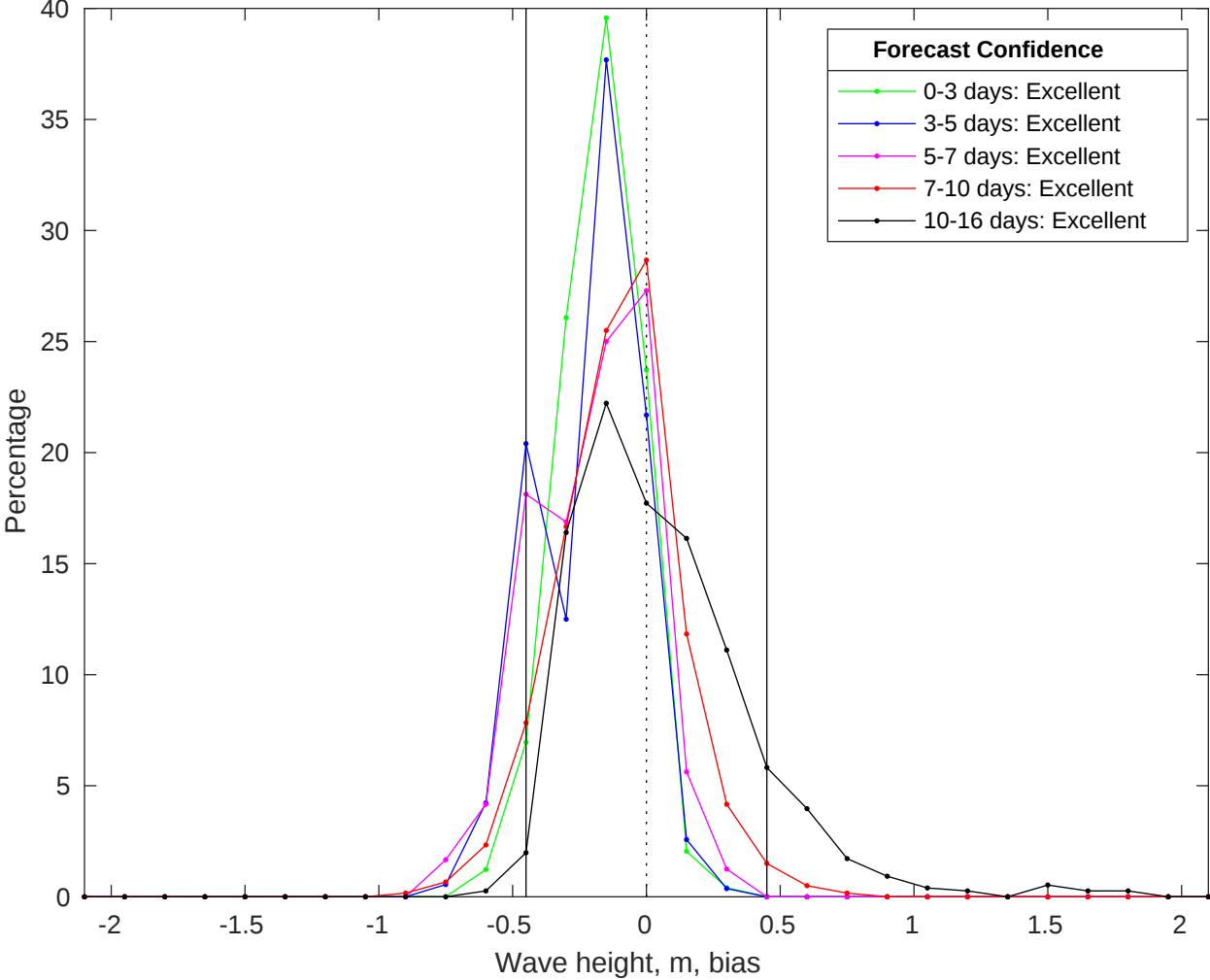
NDBC 42035 vs GFS Waves Bias Histogram: 10-Jul-2025
