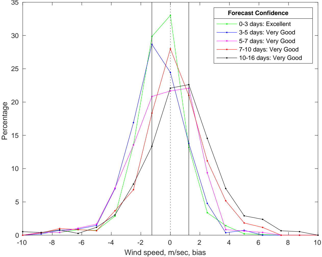
NDBC 42035 vs GFS Winds Bias Histogram: 10-Jul-2025
