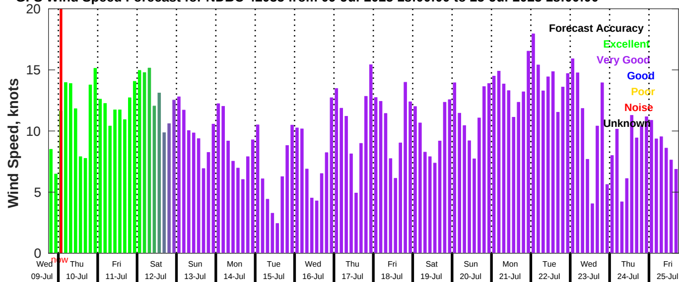
GFS Wind Speed Forecast for NDBC 42035 from 09-Jul-2025 18:00:00 to 25-Jul-2025 18:00:00
