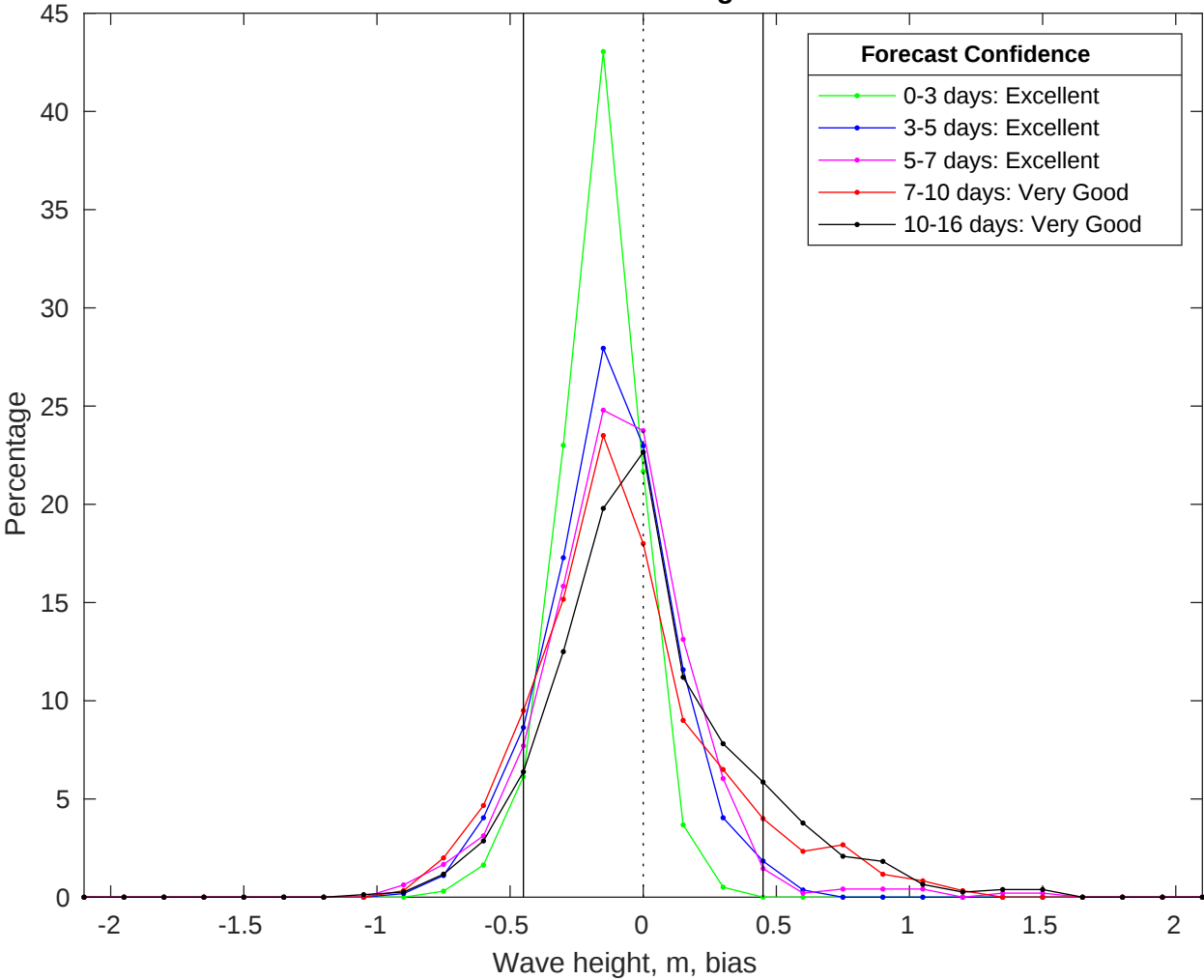
NDBC 42036 vs GFS Waves Bias Histogram: 10-Jul-2025
