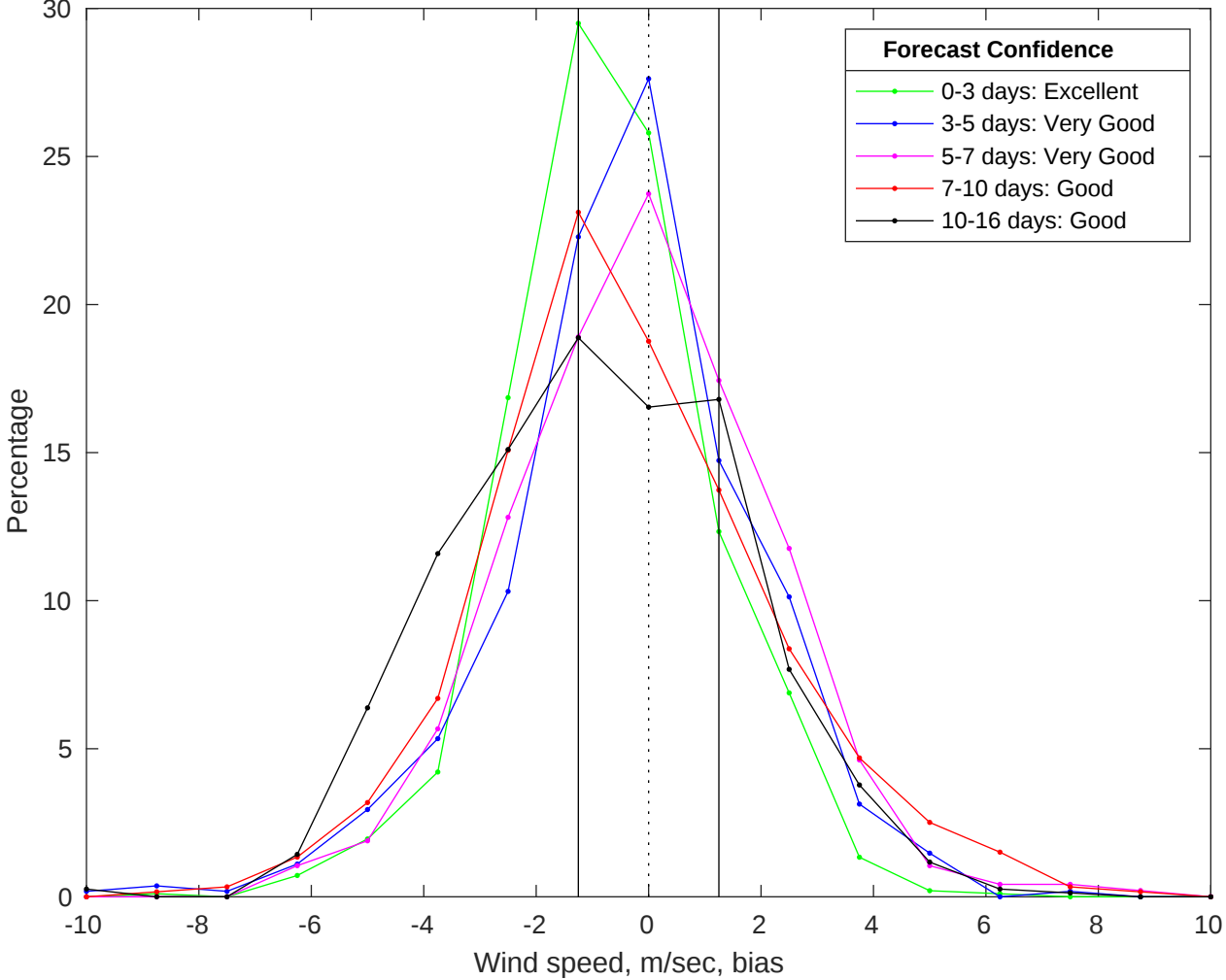
NDBC 42036 vs GFS Winds Bias Histogram: 10-Jul-2025
