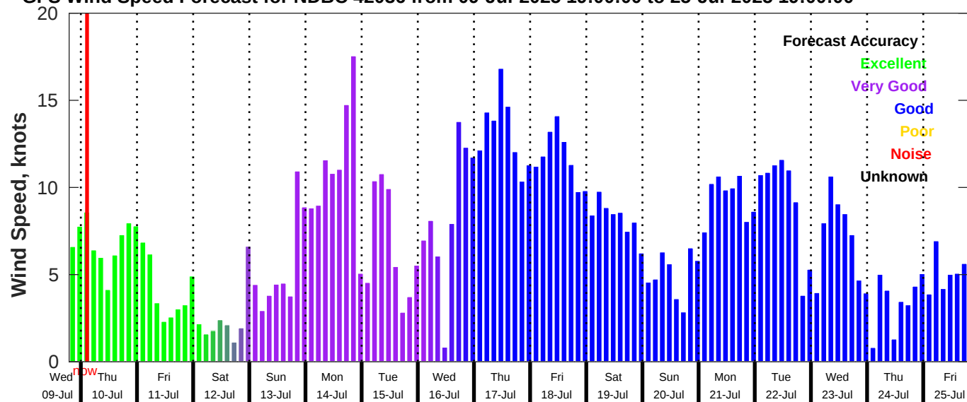
GFS Wind Speed Forecast for NDBC 42036 from 09-Jul-2025 19:00:00 to 25-Jul-2025 19:00:00
