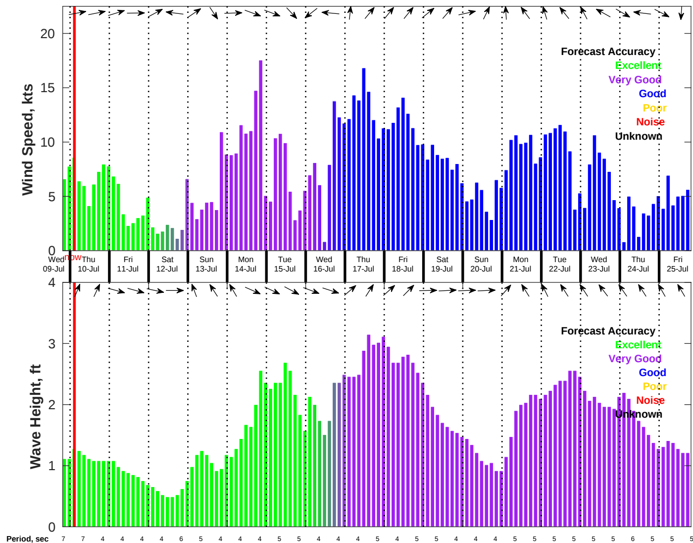
Wind & Wave Forecast for NDBC 42036 from 09-Jul-2025 19:00:00 to 25-Jul-2025 19:00:00
