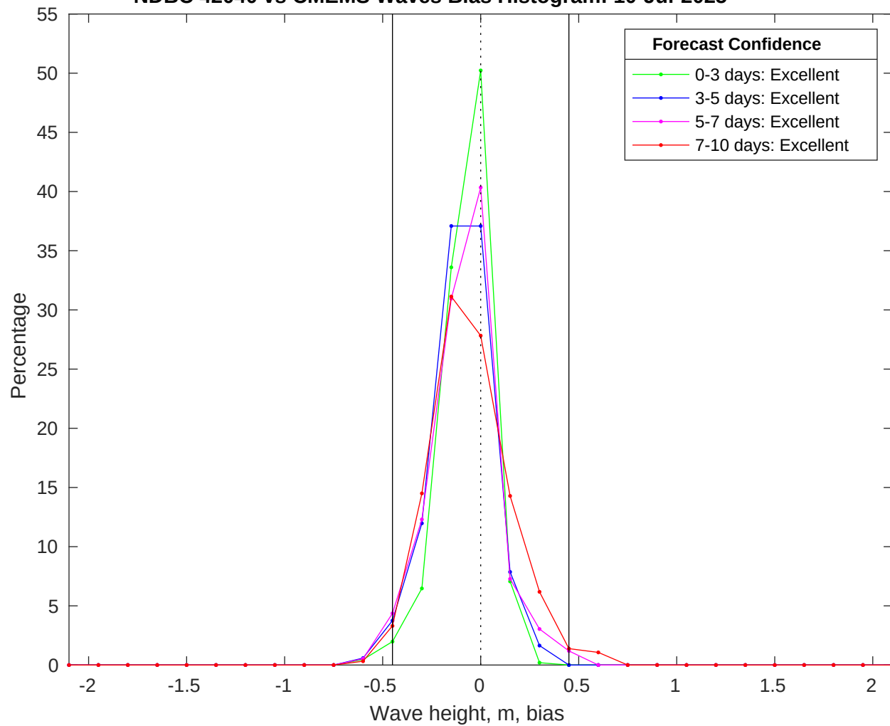
NDBC 42040 vs CMEMS Waves Bias Histogram: 10-Jul-2025
