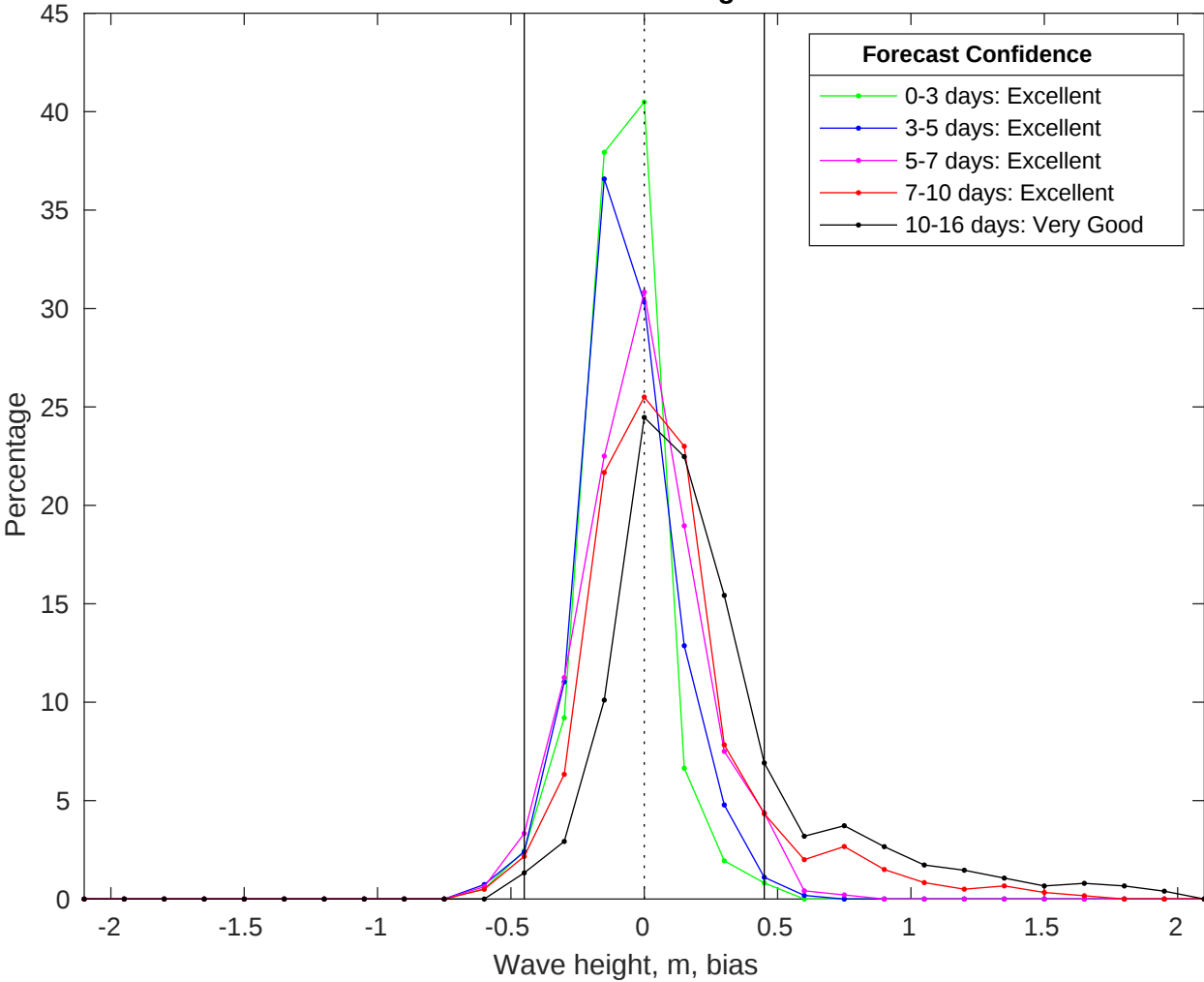
NDBC 42040 vs GFS Waves Bias Histogram: 10-Jul-2025
