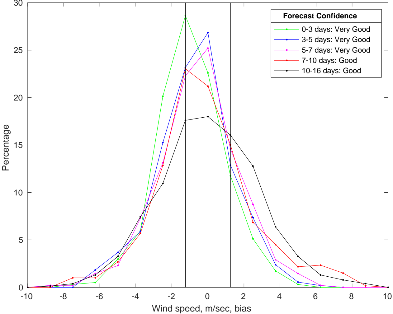
NDBC 42040 vs GFS Winds Bias Histogram: 10-Jul-2025
