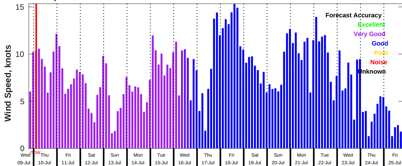
GFS Wind Speed Forecast for NDBC 42040 from 09-Jul-2025 19:00:00 to 25-Jul-2025 19:00:00
