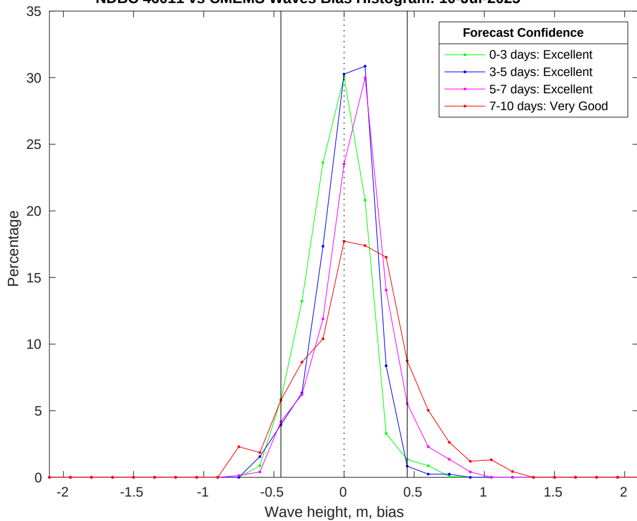
NDBC 46011 vs CMEMS Waves Bias Histogram: 10-Jul-2025
