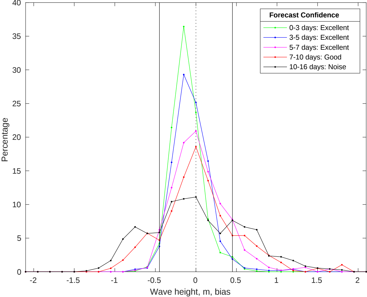
NDBC 46011 vs GFS Waves Bias Histogram: 10-Jul-2025
