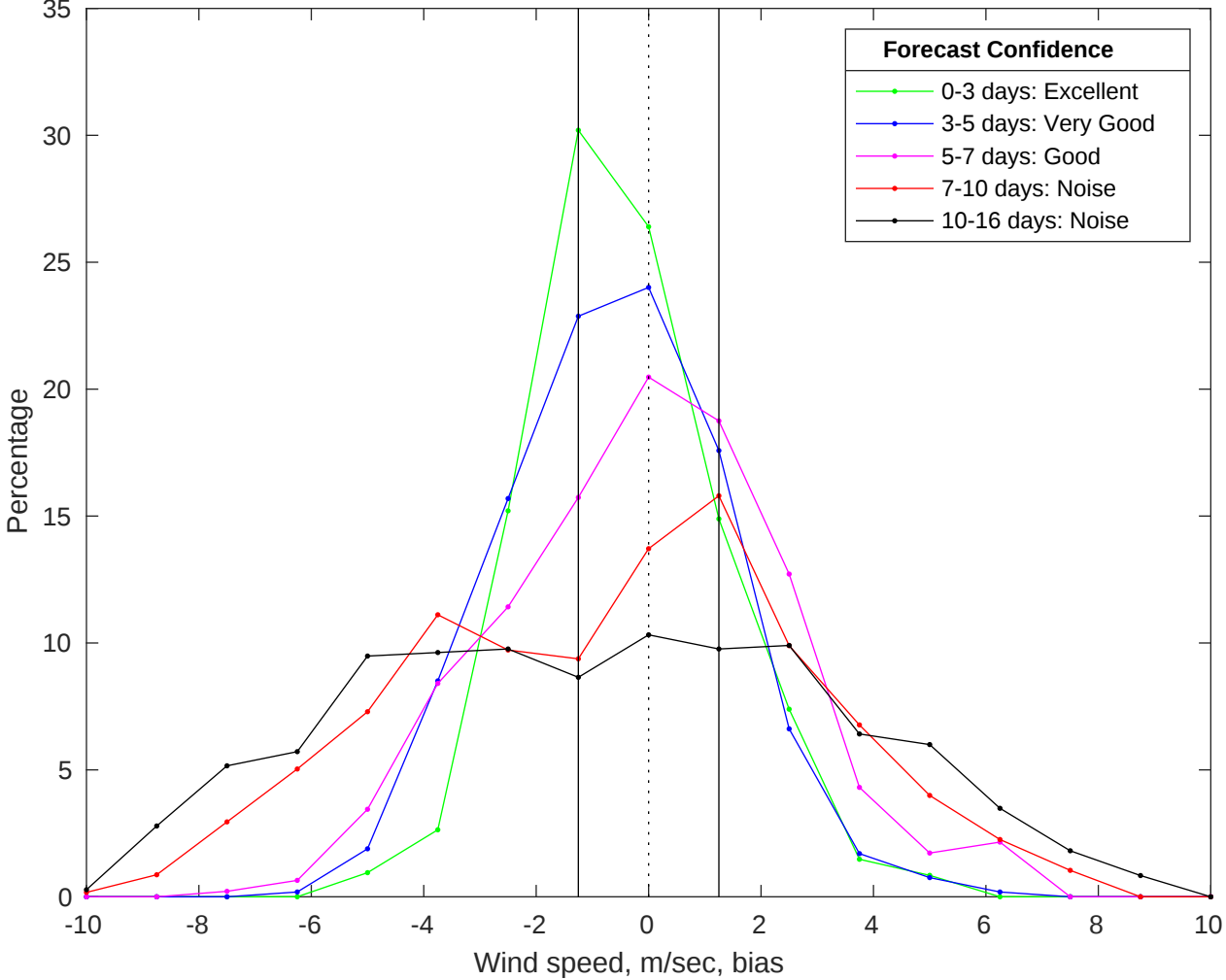
NDBC 46011 vs GFS Winds Bias Histogram: 10-Jul-2025
