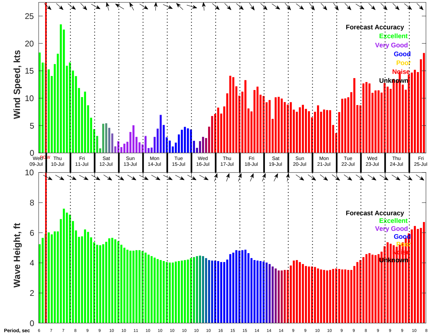
Wind & Wave Forecast for NDBC 46011 from 09-Jul-2025 16:00:00 to 25-Jul-2025 16:00:00
