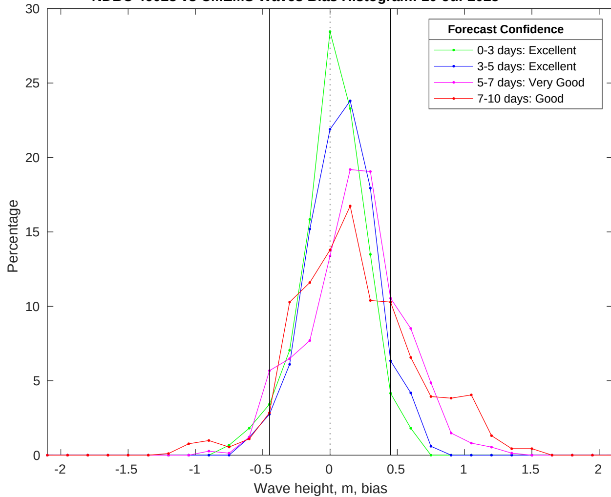
NDBC 46028 vs CMEMS Waves Bias Histogram: 10-Jul-2025
