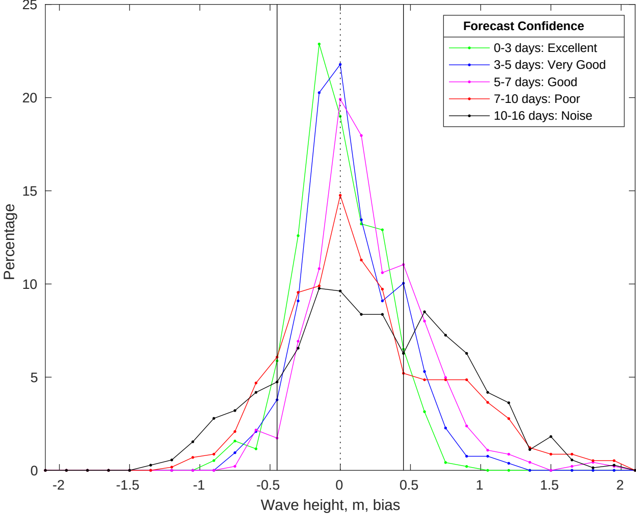
NDBC 46028 vs GFS Waves Bias Histogram: 10-Jul-2025
