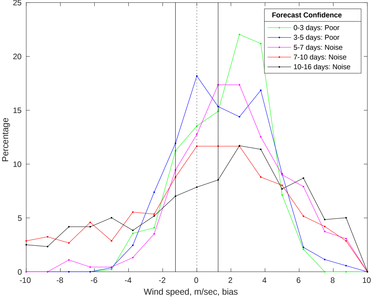
NDBC 46028 vs GFS Winds Bias Histogram: 10-Jul-2025
