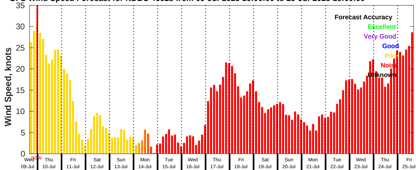
GFS Wind Speed Forecast for NDBC 46028 from 09-Jul-2025 16:00:00 to 25-Jul-2025 16:00:00
