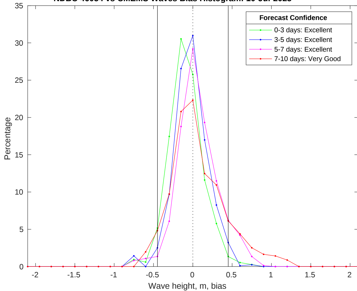
NDBC 46054 vs CMEMS Waves Bias Histogram: 10-Jul-2025
