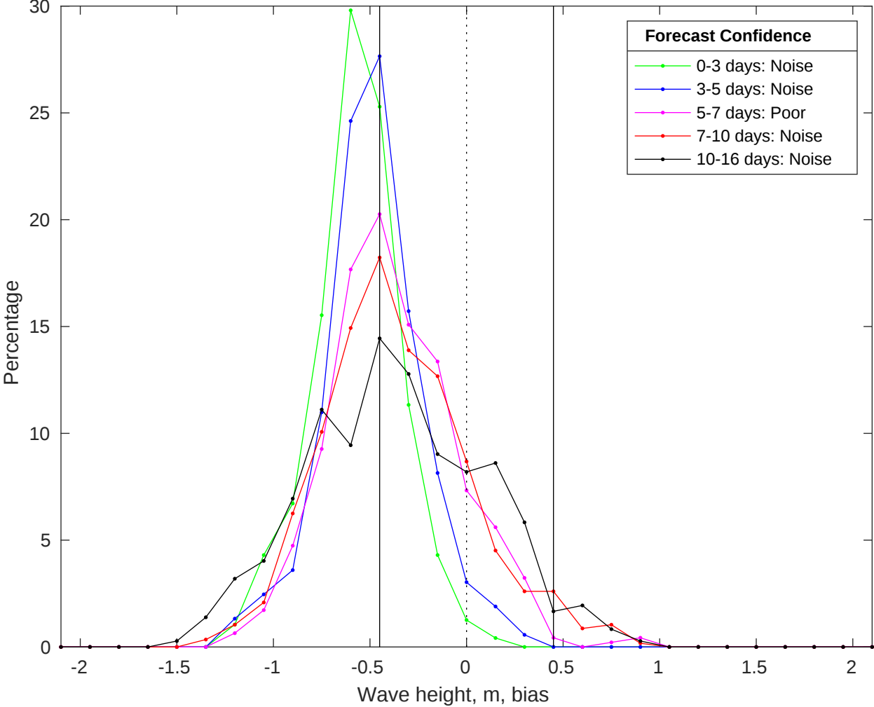
NDBC 46054 vs GFS Waves Bias Histogram: 10-Jul-2025
