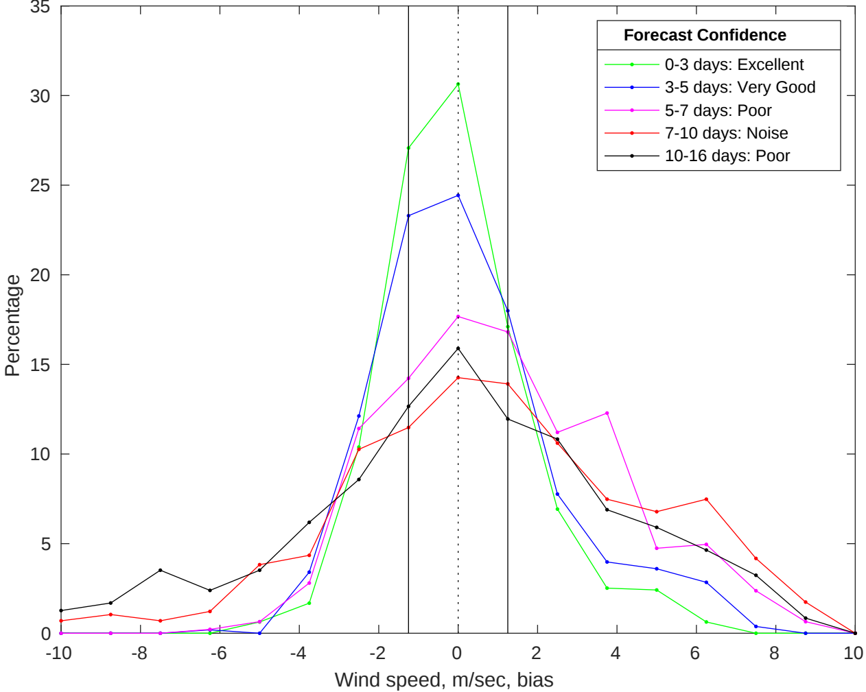
NDBC 46054 vs GFS Winds Bias Histogram: 10-Jul-2025
