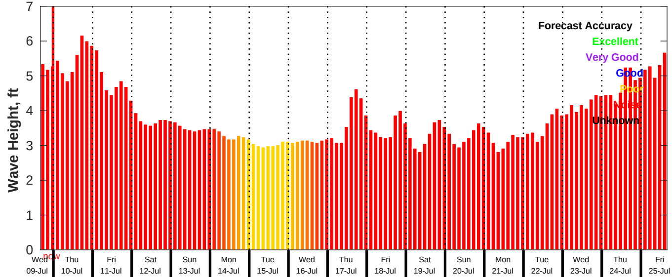
GFS Wave Forecast for NDBC 46054 from 09-Jul-2025 16:00:00 to 25-Jul-2025 16:00:00
