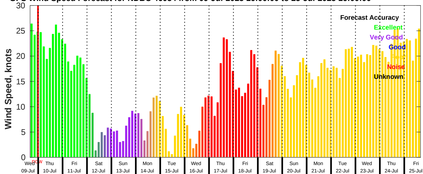
GFS Wind Speed Forecast for NDBC 46054 from 09-Jul-2025 16:00:00 to 25-Jul-2025 16:00:00
