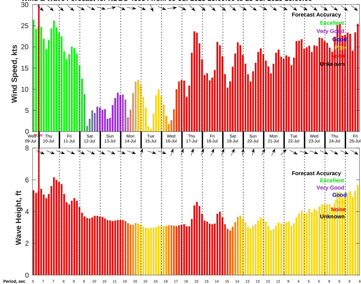
Wind & Wave Forecast for NDBC 46054 from 09-Jul-2025 16:00:00 to 25-Jul-2025 16:00:00
