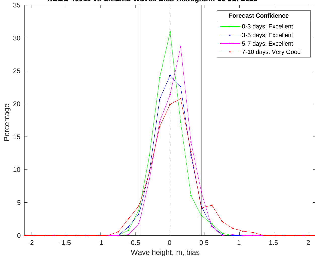
NDBC 46069 vs CMEMS Waves Bias Histogram: 10-Jul-2025
