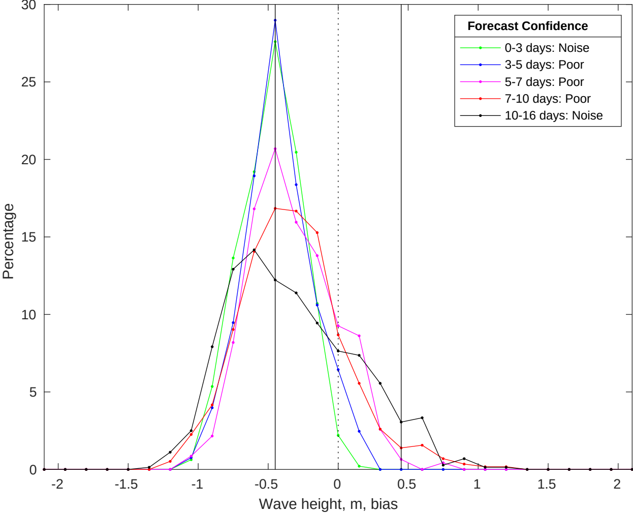
NDBC 46069 vs GFS Waves Bias Histogram: 10-Jul-2025
