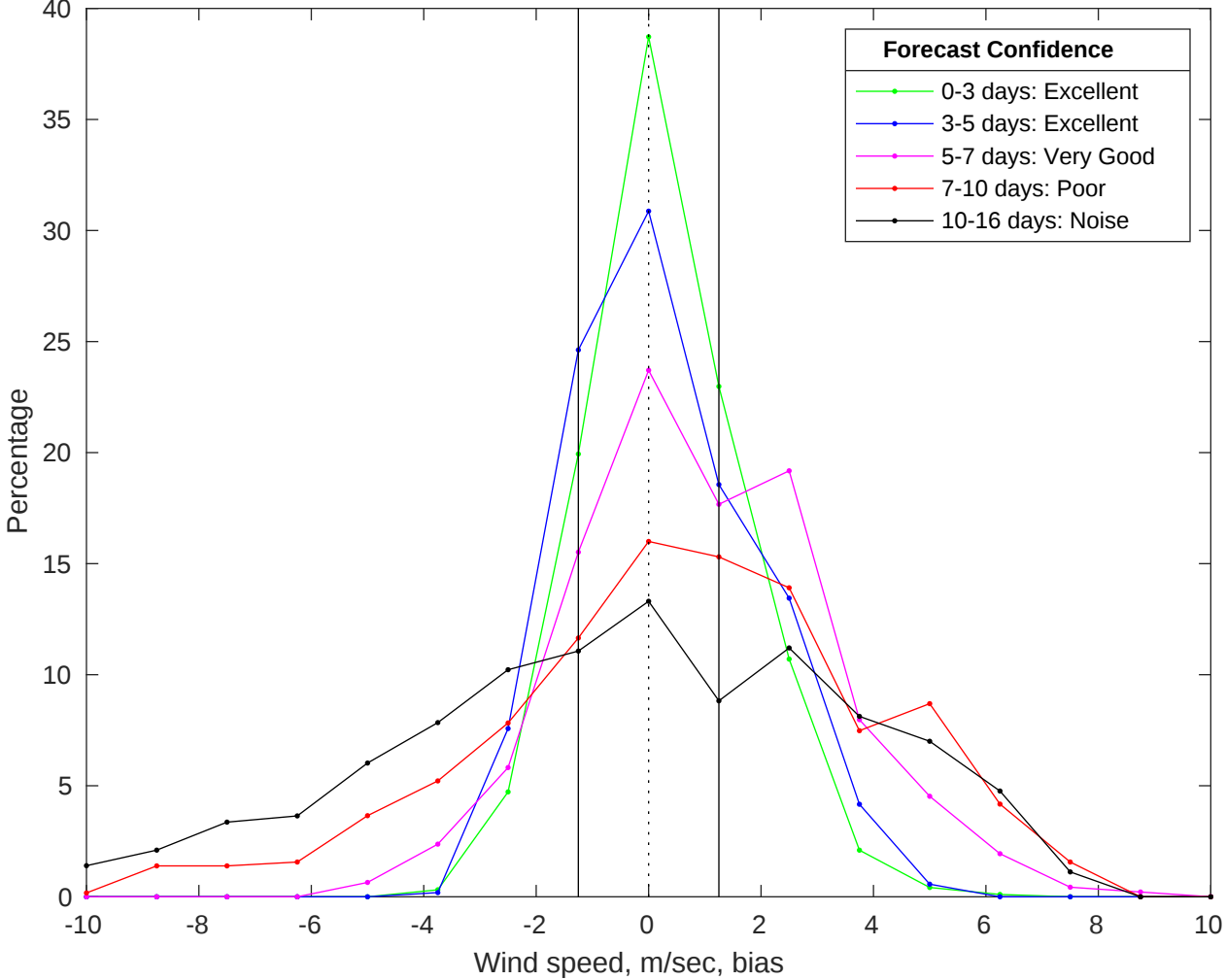
NDBC 46069 vs GFS Winds Bias Histogram: 10-Jul-2025
