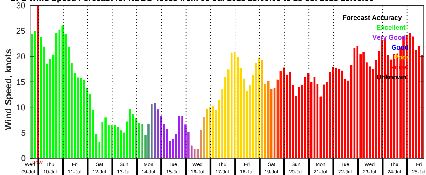
GFS Wind Speed Forecast for NDBC 46069 from 09-Jul-2025 16:00:00 to 25-Jul-2025 16:00:00
