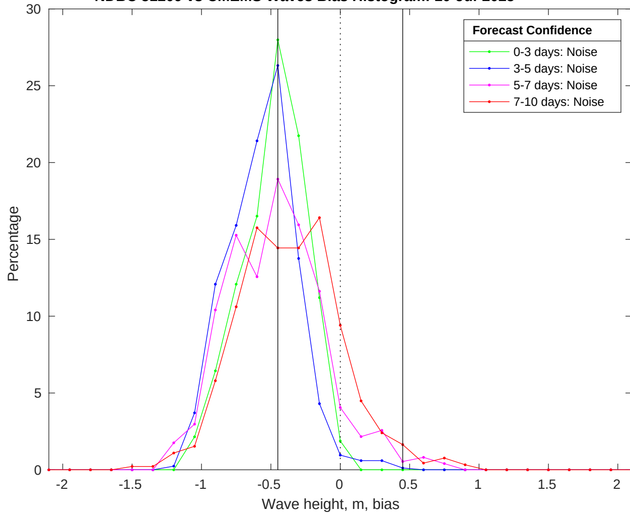
NDBC 51209 vs CMEMS Waves Bias Histogram: 10-Jul-2025
