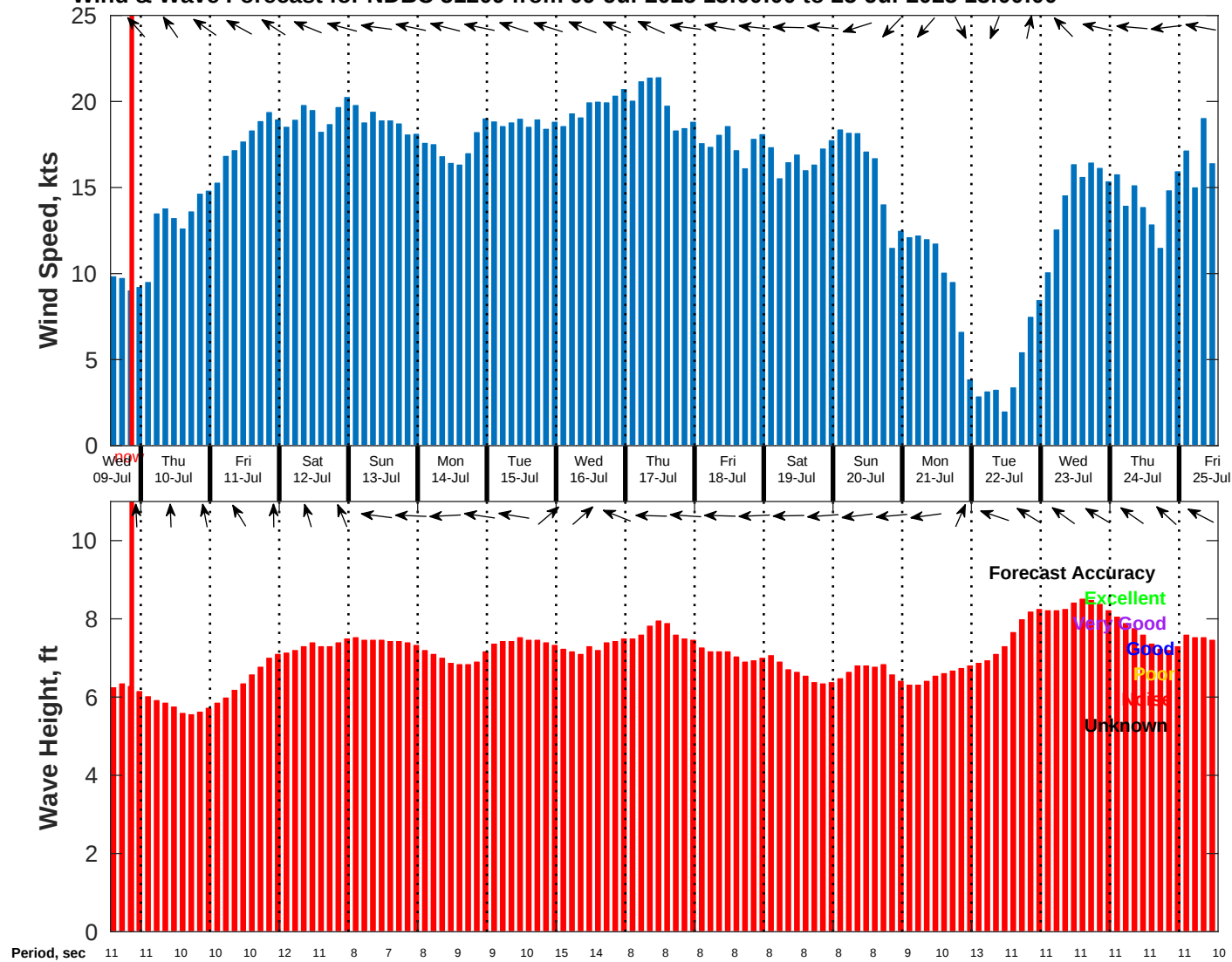
Wind & Wave Forecast for NDBC 51209 from 09-Jul-2025 13:00:00 to 25-Jul-2025 13:00:00
