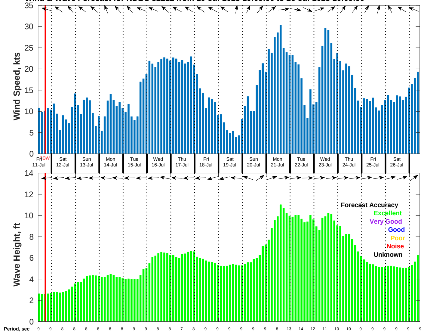
Wind & Wave Forecast for NDBC 52211 from 10-Jul-2025 10:00:00 to 26-Jul-2025 10:00:00
