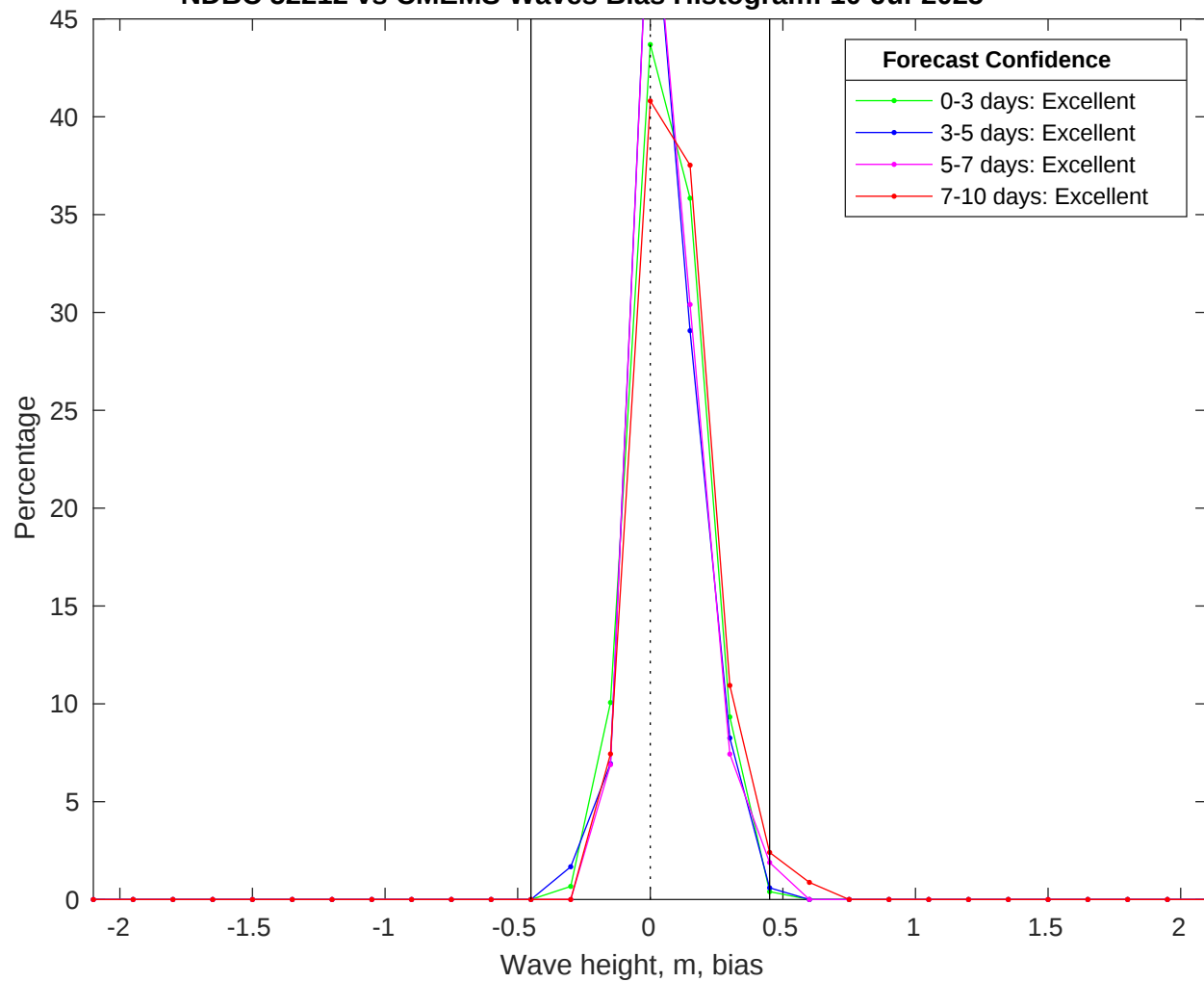
NDBC 52212 vs CMEMS Waves Bias Histogram: 10-Jul-2025
