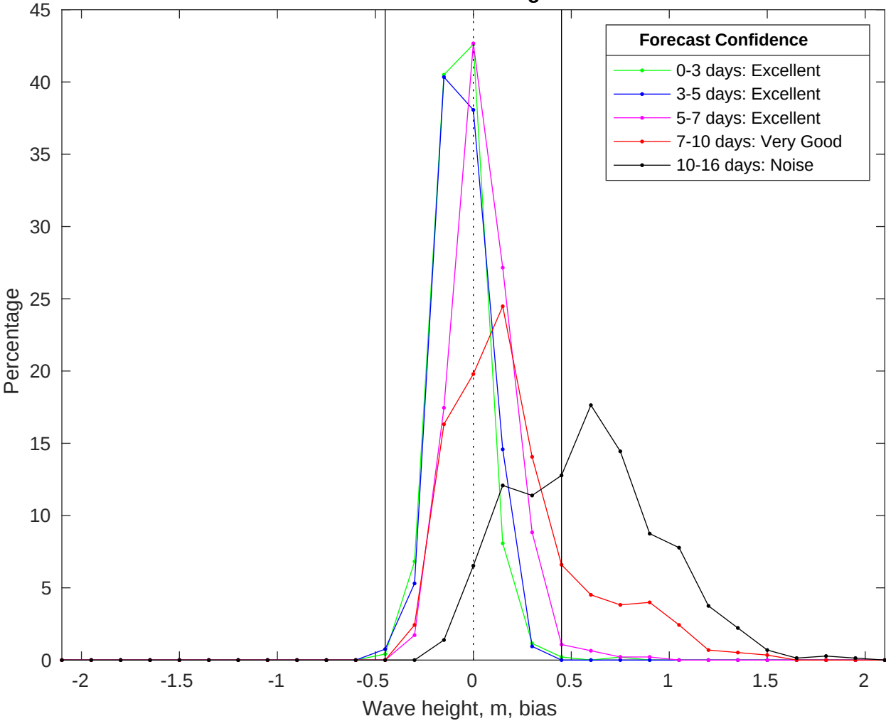
NDBC 52212 vs GFS Waves Bias Histogram: 10-Jul-2025
