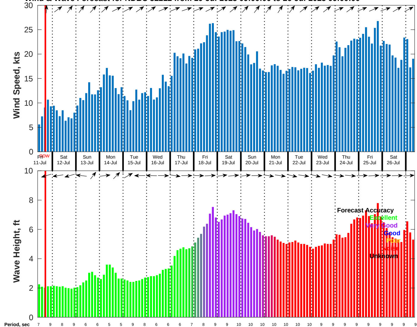
Wind & Wave Forecast for NDBC 52212 from 10-Jul-2025 09:00:00 to 26-Jul-2025 09:00:00
