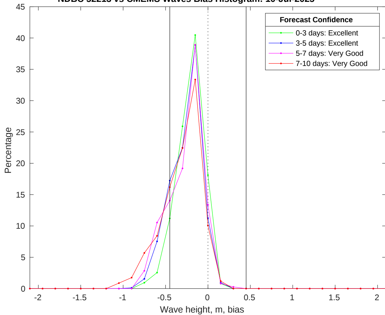
NDBC 52213 vs CMEMS Waves Bias Histogram: 10-Jul-2025
