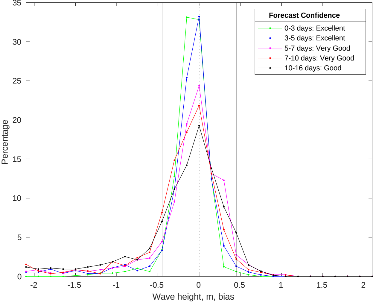
NDBC 41004 vs GFS Waves Bias Histogram: 11-Jul-2025
