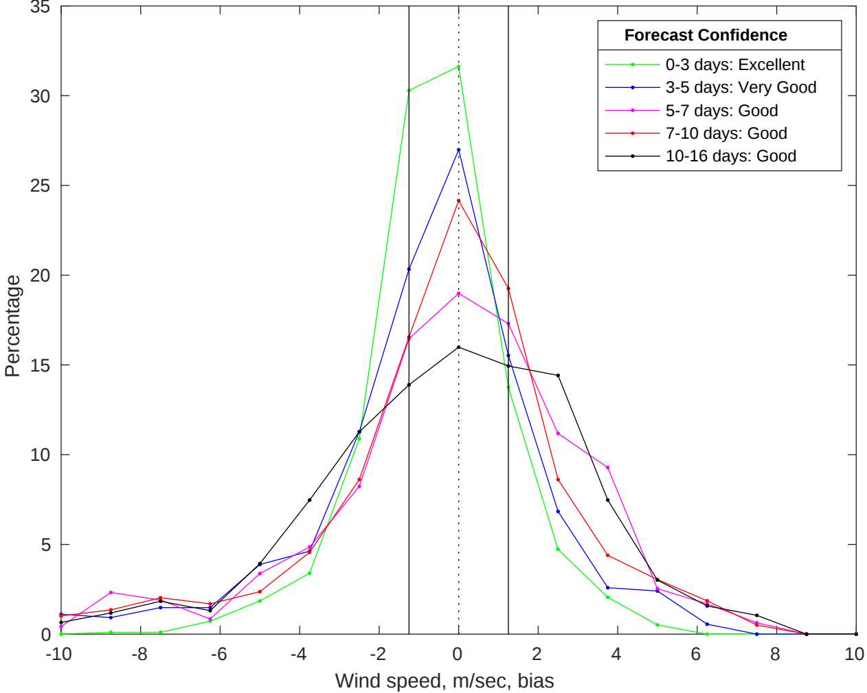
NDBC 41004 vs GFS Winds Bias Histogram: 11-Jul-2025
