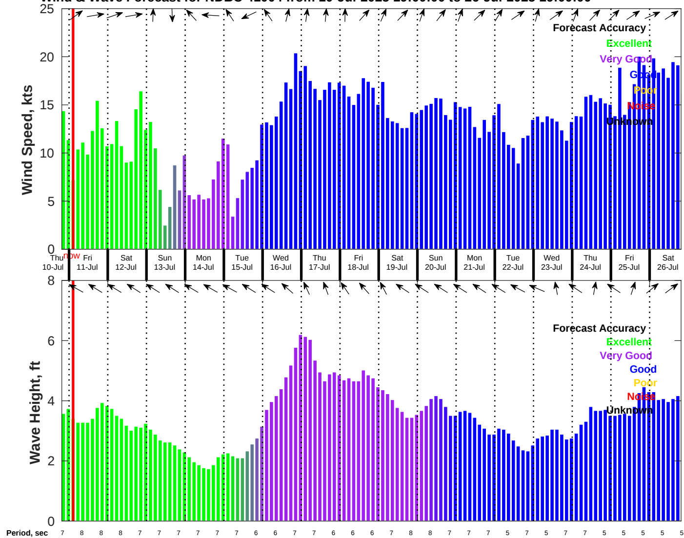
Wind & Wave Forecast for NDBC 41004 from 10-Jul-2025 19:00:00 to 26-Jul-2025 19:00:00
