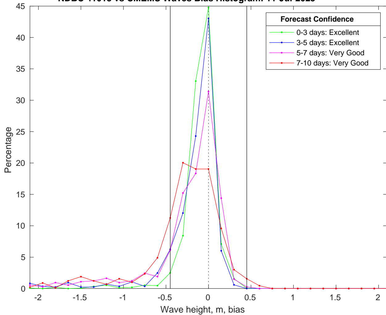
NDBC 41013 vs CMEMS Waves Bias Histogram: 11-Jul-2025
